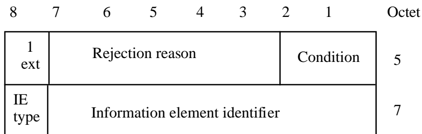
FIGURE E.2 /X.36
