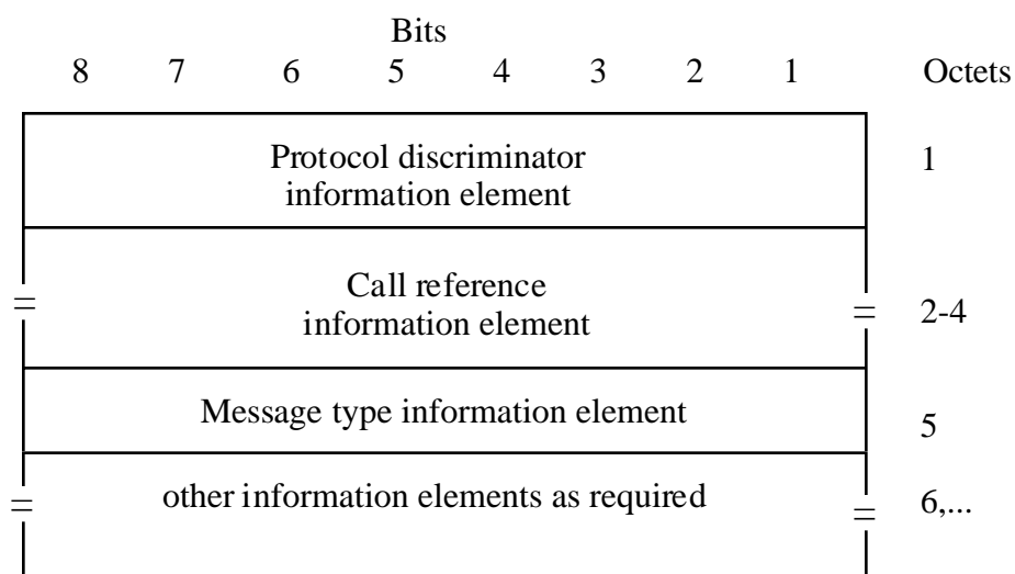
FIGURE 10.2/ X.36 General message organization example
