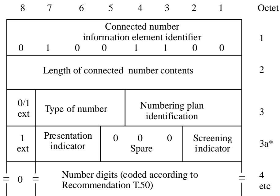
FIGURE 10.13 14/X.36 Connected number information element
