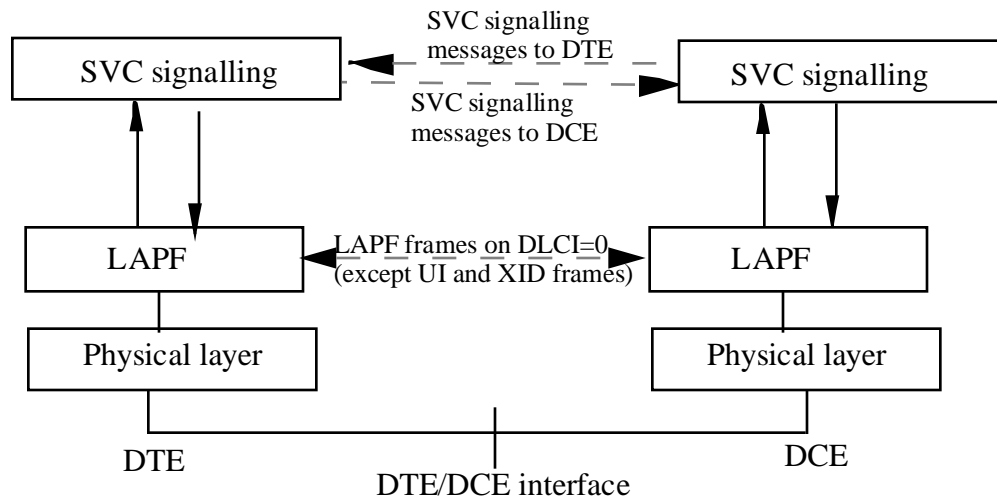
FIGURE 10.1 /X.36 DTE/DCE protocol layers for signalling
