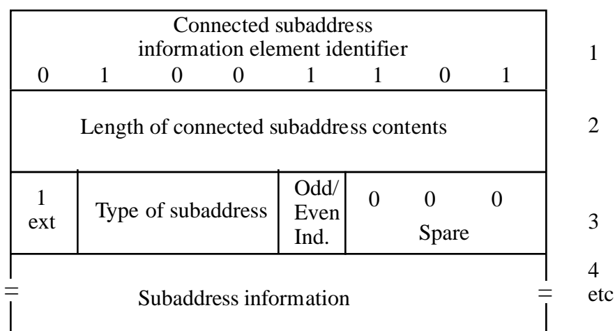
FIGURE 10.14/X.36 Connected sub-address information element
